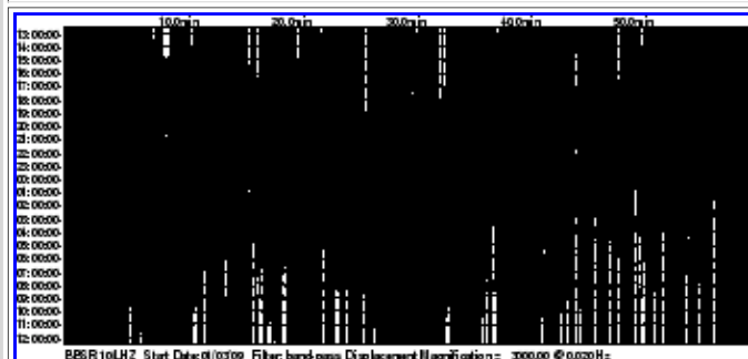
IU/CASY, Casey, Antarctica
