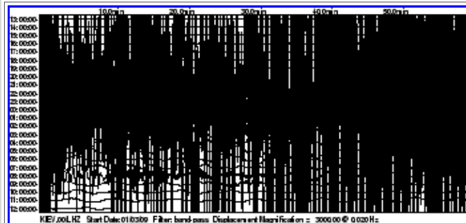
IU/KMBO, Kilima Mbogo, Kenya
